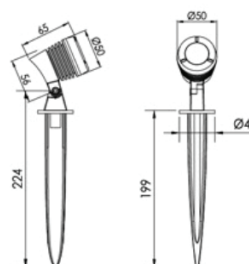
Garden Spike Accessory
